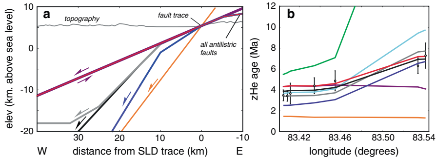
Figure 14. (a) SLD geometries tested during sensitivity testing. Orange = planar high angle. Blue = steep antilistic. Gray = rolling hinge. Black = moderate antilistic (used in main models). Red = low-angle antilistic. Purple = planar low angle. Red and purple faults have same subsurface geometry. All modeled faults daylight at mapped fault trace. No vertical exaggeration. (b) Results from sensitivity testing, presented as zHe age-longitude plot, with data as discrete points with 2-sigma error bars, and model results as lines connecting modeled ages at data point locations. Green = 1/2 modeled crustal heat production. Light blue = lower (900°C) Moho temperature. Other colors same as in Figure 14a.
