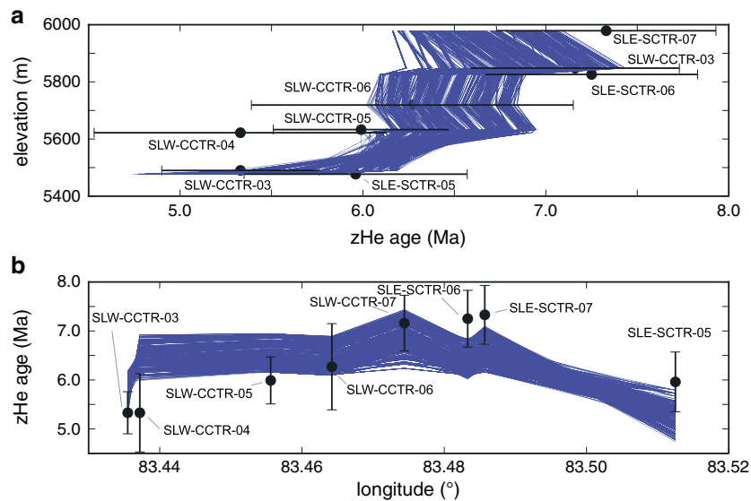
Figure 13. zHe data and Pecube model results for south transect. (a) Age versus elevation plot for observed data (black dots with 1\sigma error bars) and model results. Blue lines indicate predicted ages at each sample location for runs where all ages fit the data within 2\sigma . (b) Age versus longitude plot for same data and predicted ages. Symbology same as Figure 13a.
