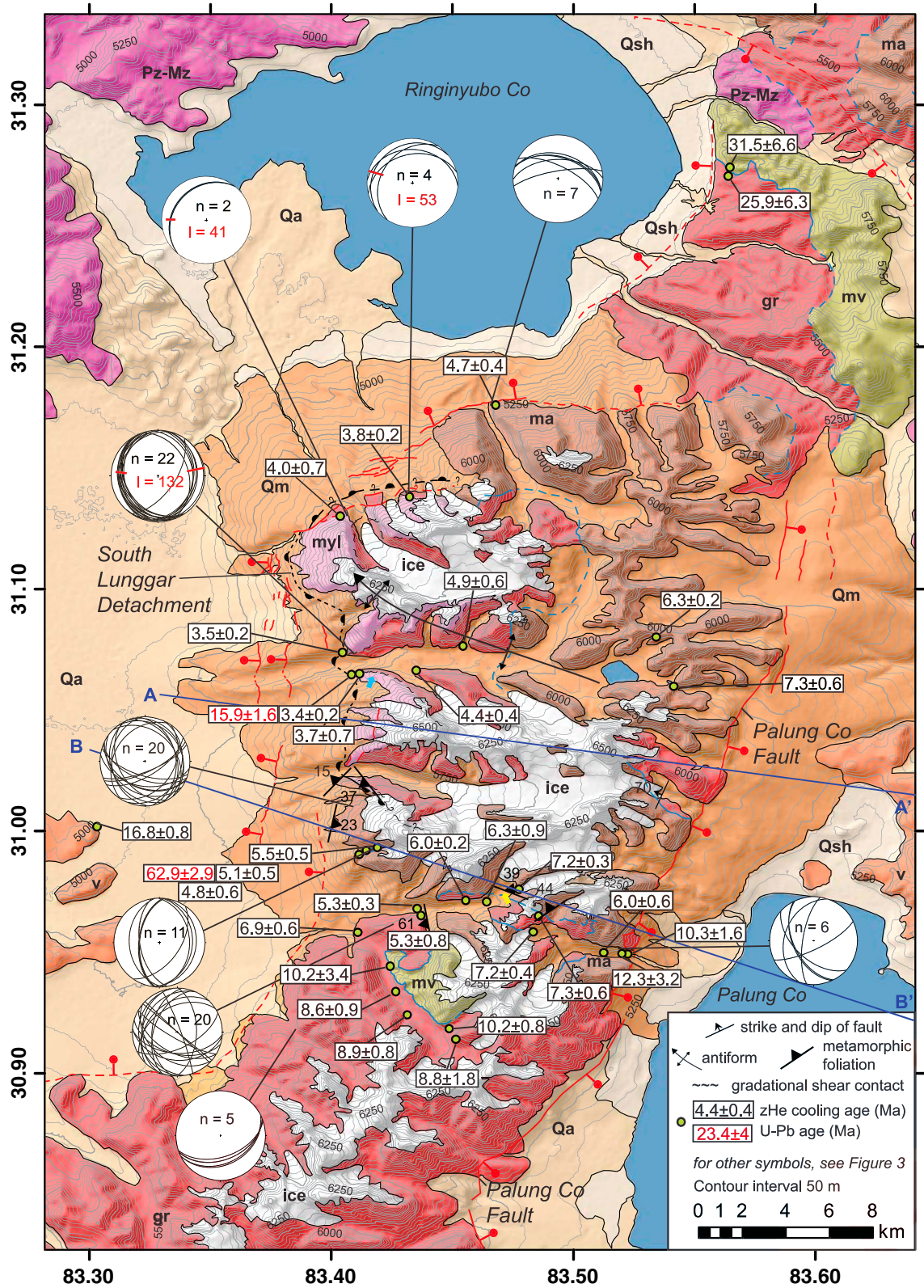
Figure 4. Geologic map of the South Lunggar rift. See Figure 3 for location. Note that cross-section lines A-A' and B-B' extend off the map to the east; see Figure 3 for full extent. On stereonets, “n” indicates the number of fault planes plotted, and “l” indicates the number of fault striations or stretching lineations measured; red lines indicate average orientation of lineations. Small blue and yellow arrows indicate position and direction field photographs (Figures 5c and 6c) were taken at. Zircon (U-Th)/He mean and 1σ errors are shown as well. Note the age for collocated samples SLE-SCTR-01 and SLE-SCTR-02 (30.94907°N, 83.52237) is the mean age for all aliquots.
