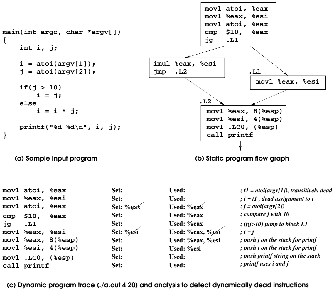
Figure 3.1. Sample example to illustrate the backward traversal algorithm to dead dynamically dead instructions
