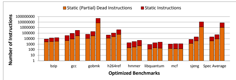
Figure 4.4. Number of static instruction instances corresponding to DDI for optimized x86 SPEC benchmarks. The three bars for each benchmark display static instructions reached without context information, with a single callee-static PC function for context information, and using the entire callee-static PC function stack as context respectively. Note, the vertical axis is plotted on a logarithmic scale
