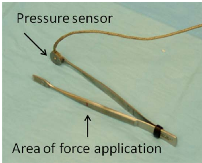
Figure 1: Photograph of the forceps device used to measure muscle compression threshold. Arrows indicate the pressure sensor (which is also the contact area with the tissue) and the site where force was applied by the examiner.
