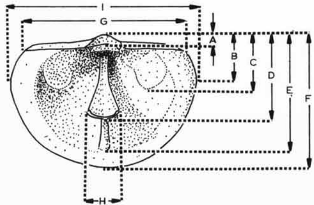
FIG. 51. Diagrammatic representation of the location of measurements on the brachial valves of Torynelasma papillosum .
