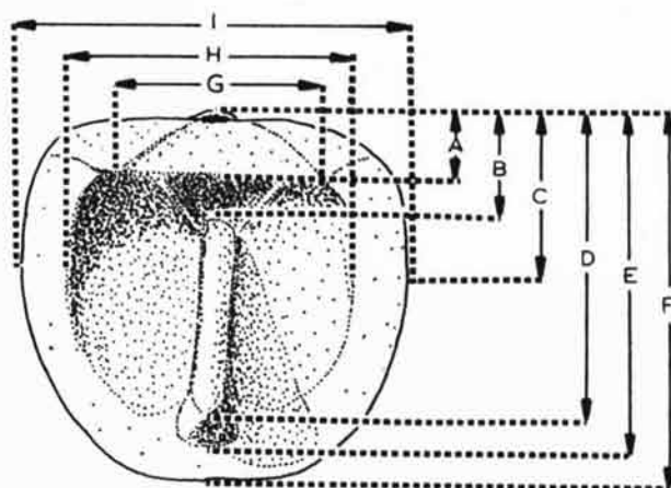
FIG. 48. Diagrammatic representation of the location of measurements on the brachial valves of Rhysotreta modesta .
