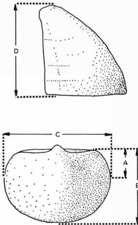
FIG. 53. Diagrammatic representation of the location of measurements on the pedicle valves of Ephippelasma spinosum .
