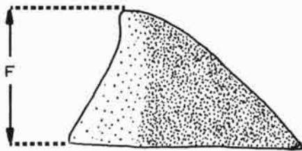
FIG. 29. Distribution of brachial valves of Conotreta mica? .
