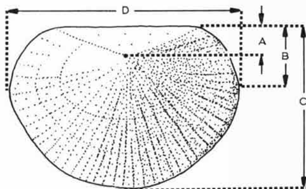
FIG. 50. Diagrammatic representation of the location of measurements on the pedicle valves of Torynelasma papillosum .
