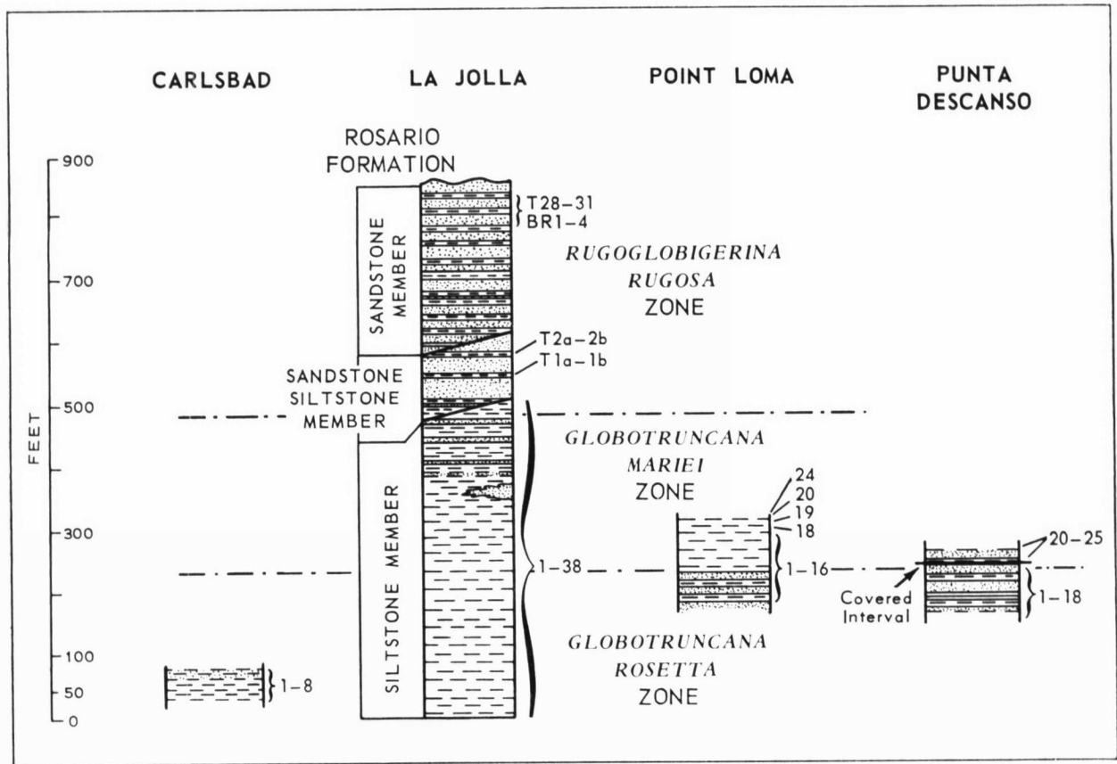
FIG. 2. Relative thicknesses and biostratigraphic zones of the Upper Cretaceous of southern California and northwestern Mexico.
