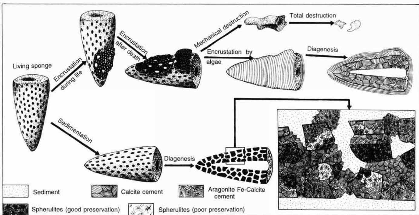
Figure 9. Diagram showing stages in diagenesis and destruction of fossil sponges in the Djebel Tebaga area. The original sponges may have been encrusted during life or after death by a variety of other sponges, algae, and miscellaneous organisms. In some beds of the area, thick coats of Archaeolithoporella obscured the sponges and locally prevented them from being mechanically destroyed. These sponges commonly underwent significant textural alteration and diagenesis. Where they were not protected and not buried in the marly sediments, the sponges may have been transported, abraded, and destroyed by mechanical processes. Other sponges, shown in the bottom of the diagram, were buried by the moderately rapid sedimentation and may have been preserved intact. They also underwent diagenesis, however, and common replacement by calcite or Fe-calcite. Various stages of diagenesis are commonly seen in single sponges at virtually every locality from which the specimens were collected.
