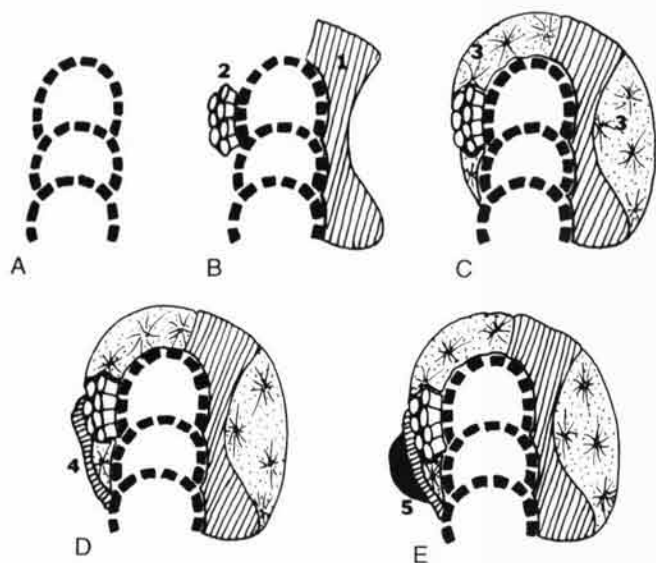
Figure 10. Encrustation succession of sponges in Upper Permian reefs of Djebel Tebaga. All figures are schematic and not to scale. A , The pioneer generation in the encrustation succession is represented by the thalamid sponge Colospongia , which was the substrate for subsequent encrustation by sponges or other organisms; B , the first generation of encrustation is represented by an undetermined organism (1), which may be algal, and the problematic and tubular organism called Permosoma (2). The time of encrusting could be the same or different for both organisms; C , after encrustation by algae and Permosoma , the next encrustation was by the prestellispongid (3), which overgrew both the pioneer host ( Colospongia ) and the encrusting algae and Permosoma . After this development, the pioneer putative colospongid was totally overgrown and could not be seen from the outside; D , a thin, sclerospongid sponge (4) next encrusted the substrate. It has very small tubes and partly or totally encrusted the Permosoma or the Prestellispongia , so that only the sclerosponge could be seen from the outside; E , finally, the last generation of encrustation (5) was a thin sheet of an undetermined organism, which grew over part of the sheet of the sclerosponge.
