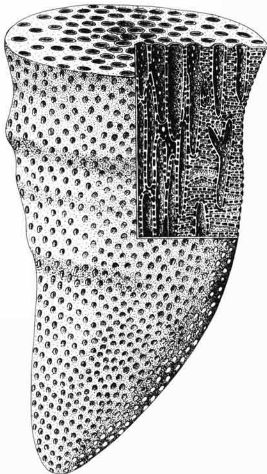
Figure 32. A reconstruction of Medenina laterala new species. The vertical section shows the loosely packed vertical canals near the periphery of the sponge and horizontal skeletal elements between them. Both walls of the canals and the horizontal elements have numerous small pores. The transverse cross section shows exhalant tubes concentrated in the axial area of the sponge (schematic, not to scale).
