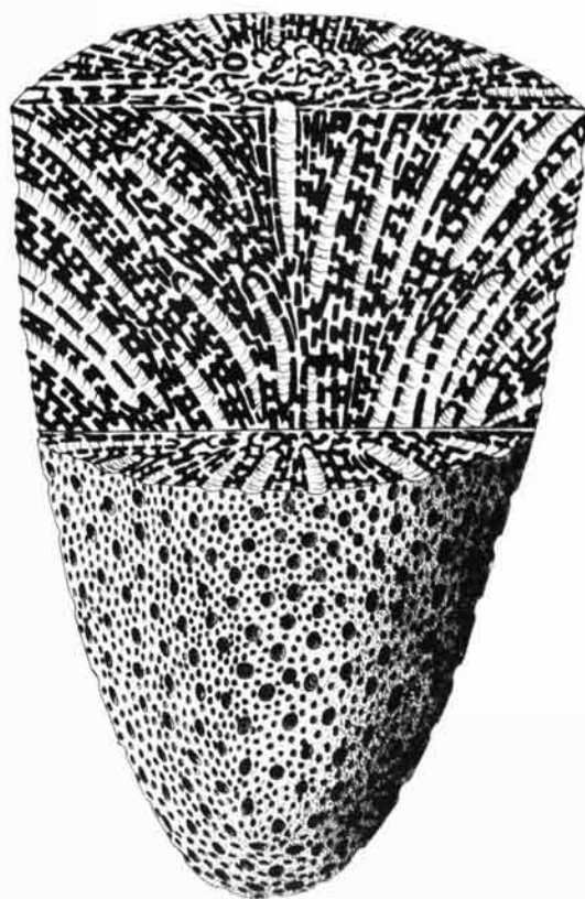
Figure 15. Reconstructions of longitudinal and transverse sections of Radiotrabeulopora maokoui Fan, Rigby, and Zhang, 1991. The large exhalant canals diverge upward within the sponge, but they appear as radially arranged openings in transverse sections, especially in the outer part of the sponge. In transverse sections the axial part appears composed mainly of fibers and only a few inhalant canals. Spaces between the canals are filled with fibers that are oriented upward and outward within the sponge, parallel to the exhalant canals. Small inhalant pores on the surface of the sponge extend inward as inhalant canals between the fibrous structures. In longitudinal section the large exhalant canals appear upwardly divergent, and the spaces between them are filled with skeletal fibers arranged parallel to the exhalant canals (schematic, not to scale).
