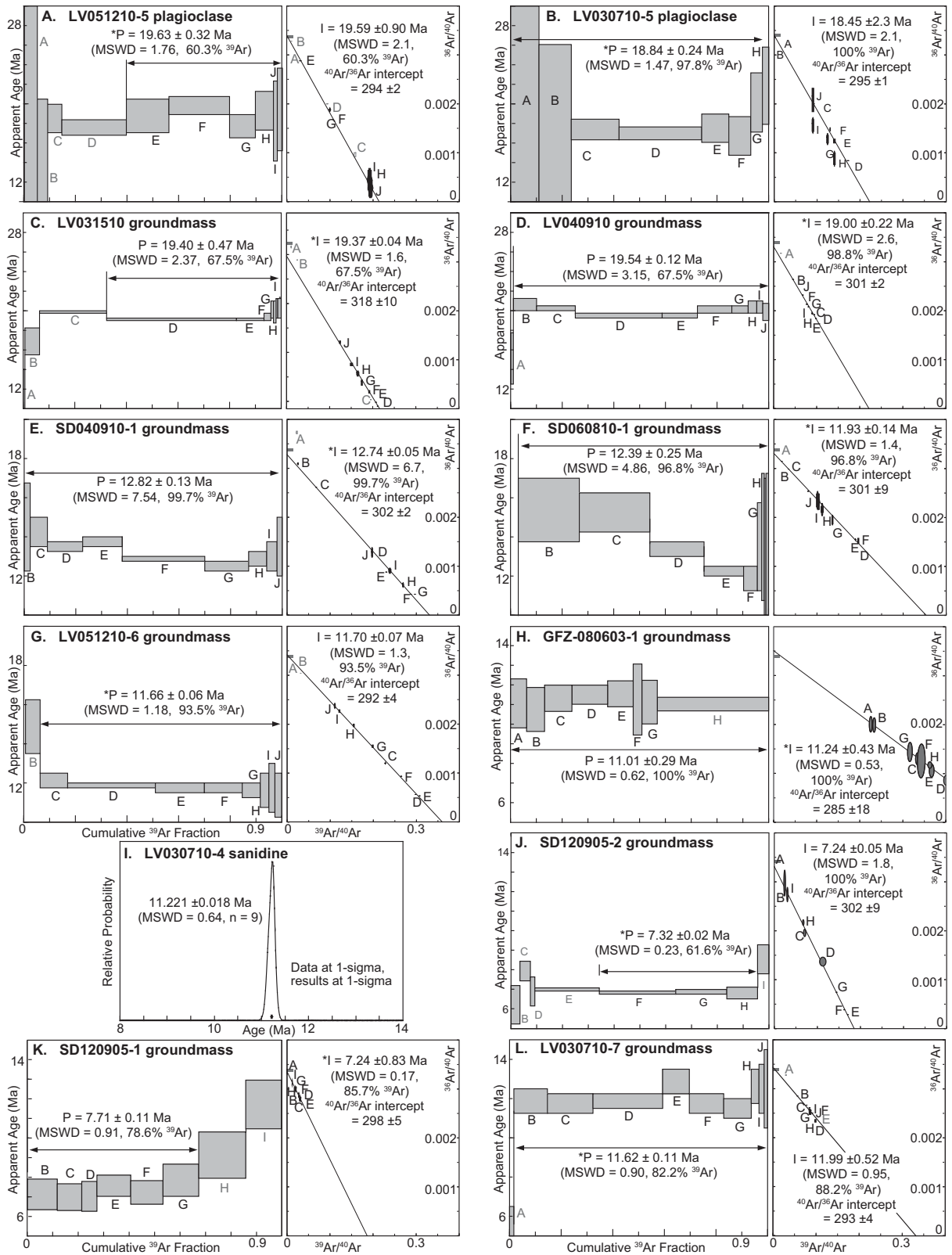
Figure 4. Plots of plateau diagrams and inverse isochrons for step-heating ^{40}\text{Ar}/^{39}\text{Ar} analyses of our new samples, except I, which is a frequency plot of analyses of sanidine (MSWD—mean square of weighted deviates). Interpreted ages are reported using plateau (P) and inverse isochron (I) methods with the preferred age denoted by (*). Double-headed arrows indicate the steps included in the plateau age. Fraction labels (i.e., A, B, C, etc.) in gray were not used in the age interpretation. The small gray box on the inverse isochron plots denotes the value of atmospheric argon with ^{40}\text{Ar}/^{36}\text{Ar} of 295.5.
