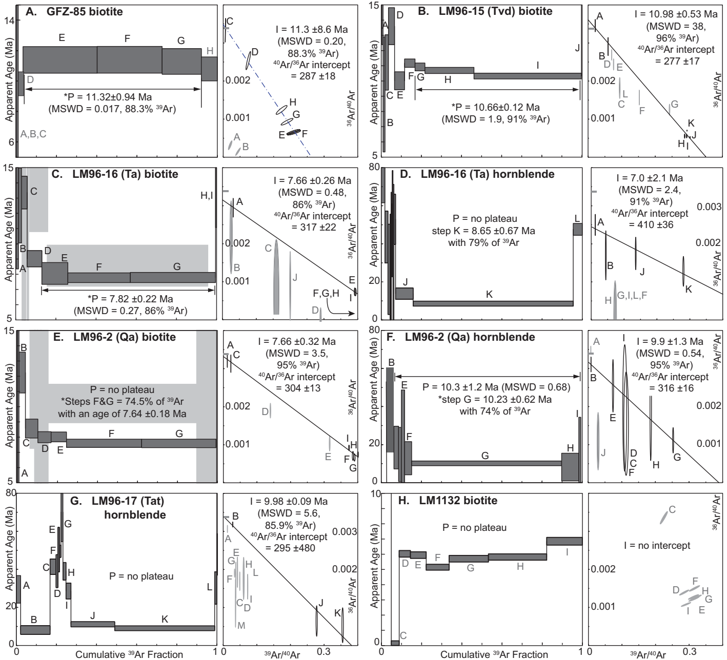
Figure 6. Plots of plateau diagrams and inverse isochrons for step-heating ^{40}\text{Ar}/^{39}\text{Ar} analyses of the reinterpreted samples from Smith et al. (2002). See Figure 4 for symbol and abbreviation explanations. The gray blocks on C and E are the corresponding hornblende data for each sample.
