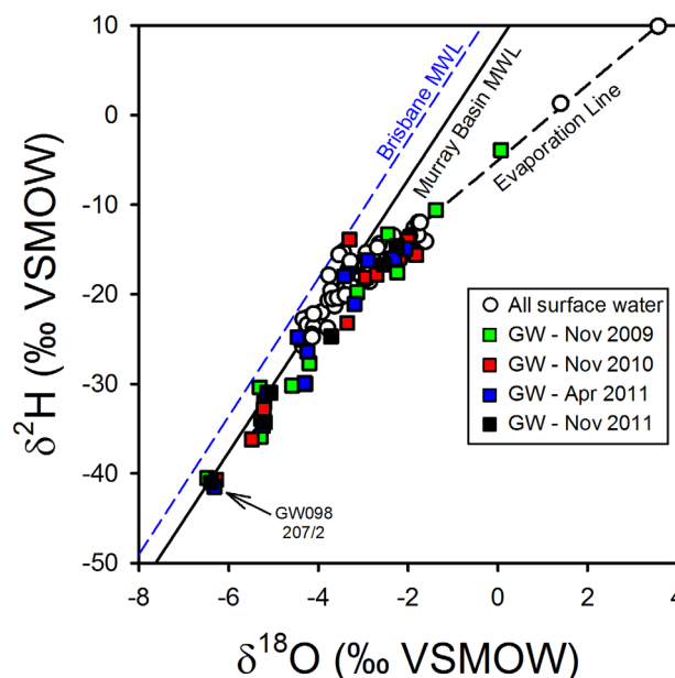
Figure 7. \delta^2\text{H} - \delta^{18}\text{O} plot for all surface and groundwater samples collected during the study. Also shown is the Brisbane Meteoric Water Line ( \delta^2\text{H} = 7.6 \cdot \delta^{18}\text{O} + 13 ) [Crosbie et al., 2012], the Murray Basin Meteoric Water Line ( \delta^2\text{H} = 7.6 \cdot \delta^{18}\text{O} + 8 ) [Simpson and Herczeg, 1991] and the evaporation line for the surface water samples ( \delta^2\text{H} = 4.3 \cdot \delta^{18}\text{O} - 5.1 ).
