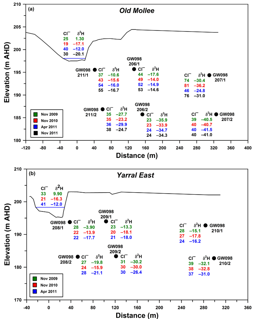
Figure 6. Chloride concentration (mg L -1 ) and δ 2 H (‰ VSMOW) during the four sampling campaigns (there was no sampling at Yarral East on November 2011). (a) Old Mollee and (b) Yarral East.
