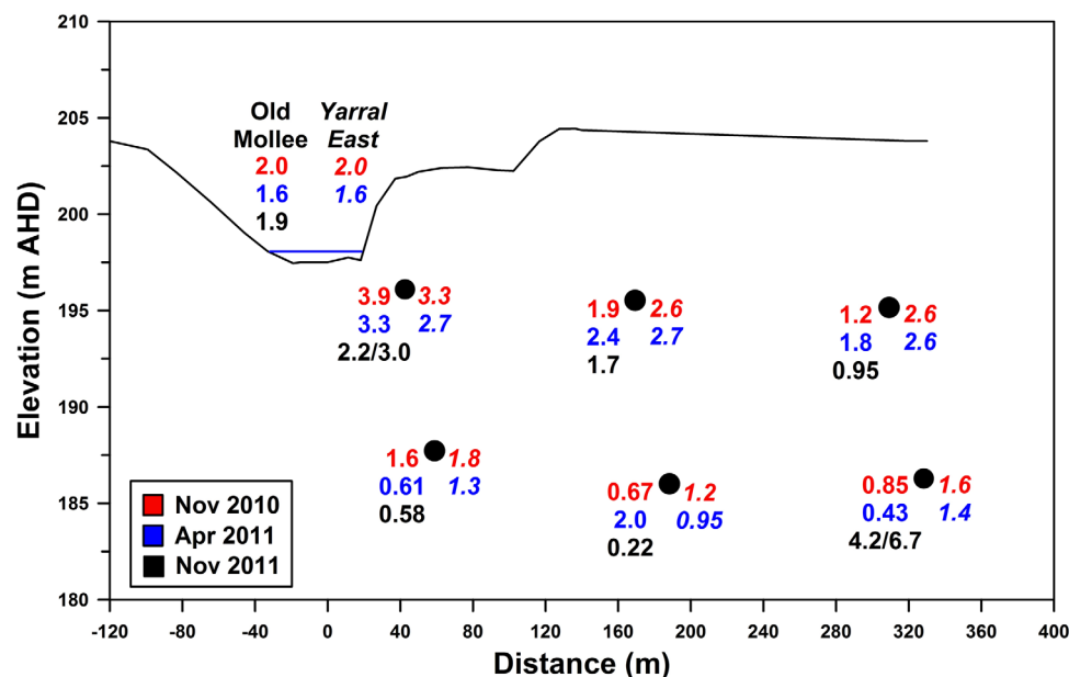
Figure 8. SF 6 concentrations (fmol kg -1 ) in surface and groundwater at Old Mollee and Yarral East on three different sampling campaigns (cross section for Old Mollee shown).
