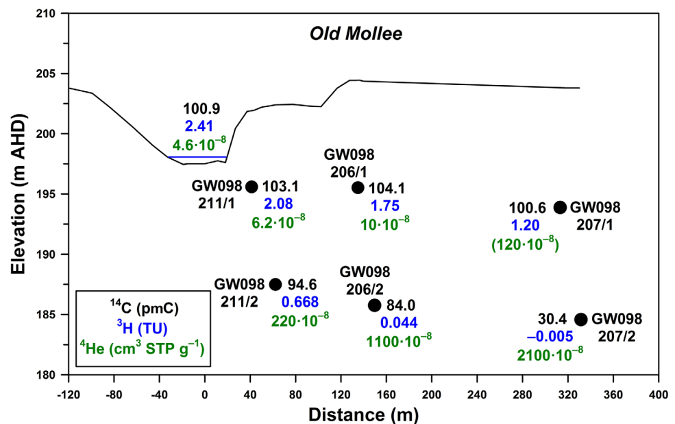
Figure 10. Carbon-14, ^3\text{H} , and ^4\text{He} concentrations at Old Mollee on November 2011, except for ^4\text{He} at bore GW098207/1 which was the average from the November 2010 and April 2011 samplings.
