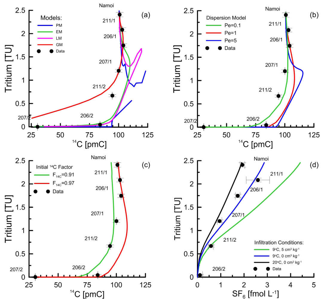
Figure 11. Evaluation of the ^3\text{H} , ^{14}\text{C} , and \text{SF}_6 data using lumped parameter models. (a) Comparison of different types of ^3\text{H}/^{14}\text{C} models (PM, Piston Flow; EM, Exponential; LM, Linear; GM, Gamma) [Suckow, 2012], (b) ^3\text{H}/^{14}\text{C} dispersion models for different Pe values, (c) Effects of variations in the ^{14}\text{C} atmospheric input function correction factor ( F_{14\text{C}} ) for a DM model with Pe = 0.1 (green) and 1 (red), and (d) \text{SF}_6 concentrations evaluated with a ^3\text{H}/\text{SF}_6 Dispersion Model with Pe = 0.5 , showing that the range in excess air and in temperature at recharge estimated for the aquifer can account for the observed variations in \text{SF}_6 concentrations in shallow piezometers.
