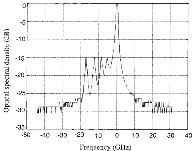
Fig. 3. Measured OSSB spectrum with four subcarrier channels.
